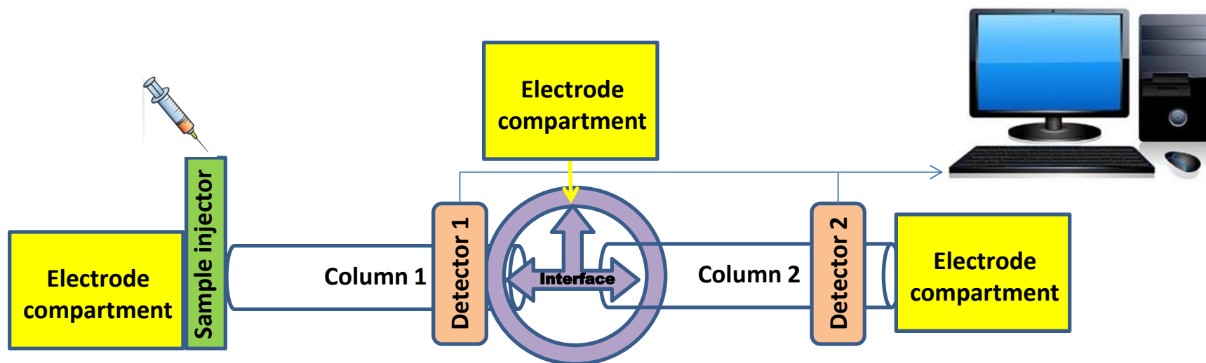
2D-CE instrumental arrangement
