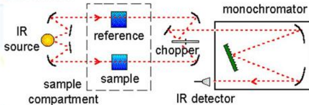
Schematic of a dispersive (double beam) IR spectrometer
