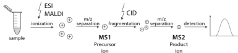
Tandem mass spectrometry (MS/MS) (basic procedure)
