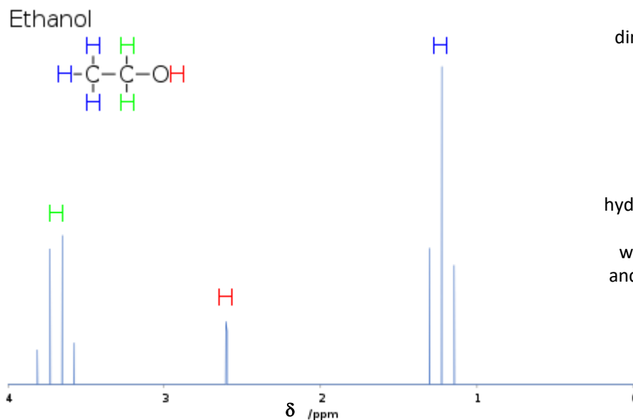
NMR spectrum
